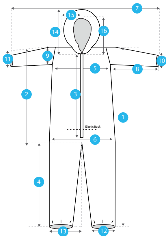
Antistatic Disposable Hooded Coverall Type 5/6
